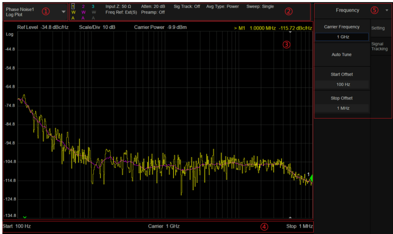
Figure 3-1 Operation interface of phase noise analysis function
