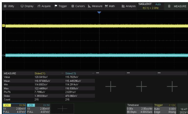
12-bit resolution shows you more details and less noise on the waveform
