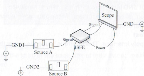
Use ISFE to isolate the channels of scope
